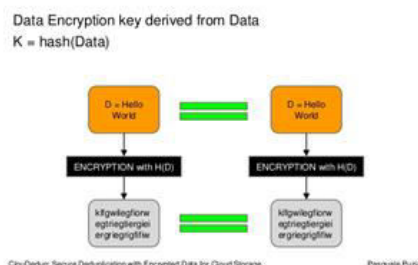
Fig 4.Convergent Encryption
